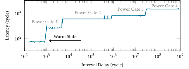
Fig. 1: Performance States of AMX due to Power Gating
