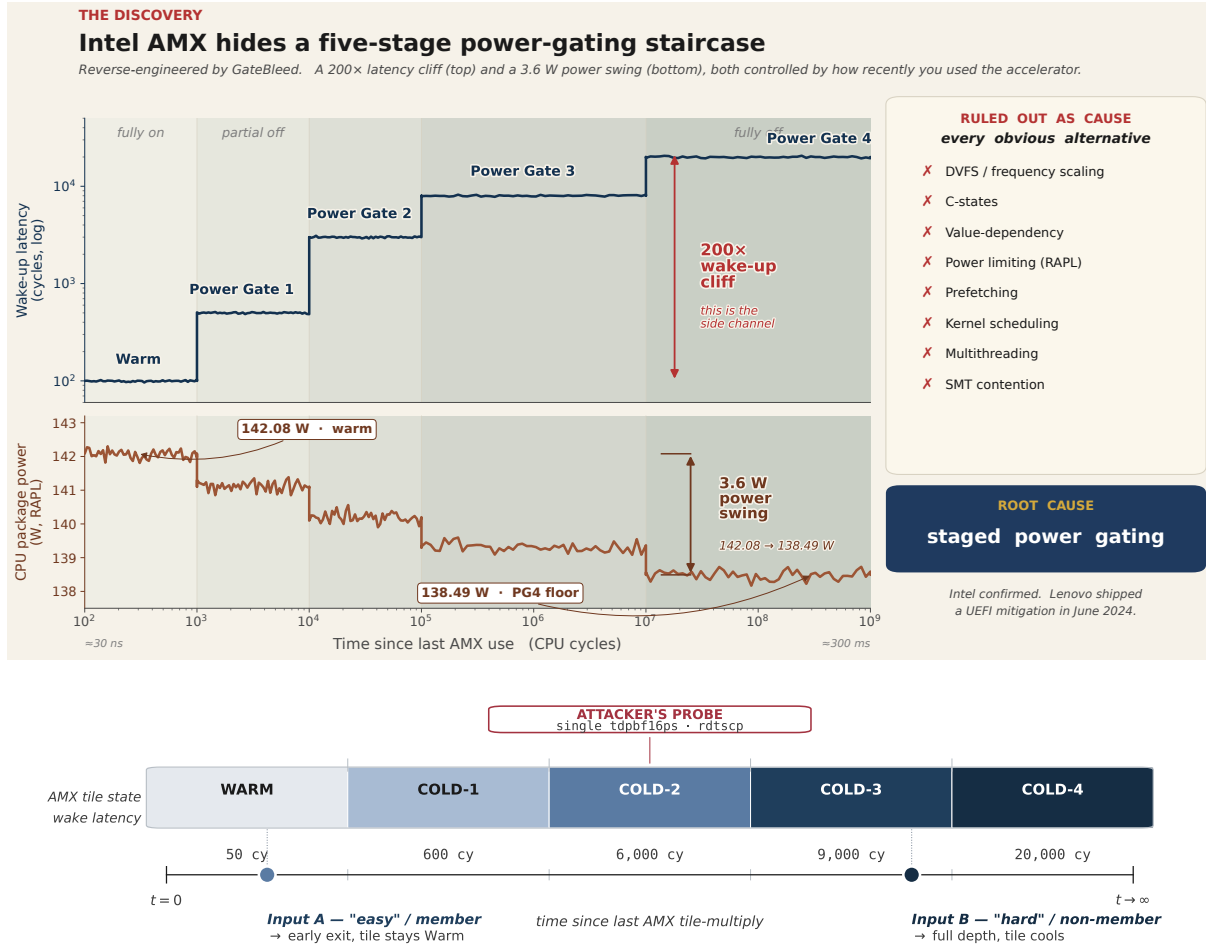
FIGURE 2: Performance states of Intel AMX due to staged power gating. Top: wake-up latency staircase versus time since the last AMX use, with a 200× latency gap across five plateaus reaching ~ 20,000 cycles at the deepest stage. Middle: CPU package power (W, RAPL) on the same x-axis; the 3.6 W swing from 142.08 to 138.49 W is the corroborating signal. Bottom: a single attacker probe ( tdpbf16ps · rdtscp ) reads the plateau the accelerator occupies, encoded by the input the model processed.
