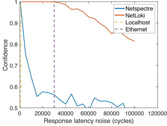
Fig. 4. Noise resilience.
